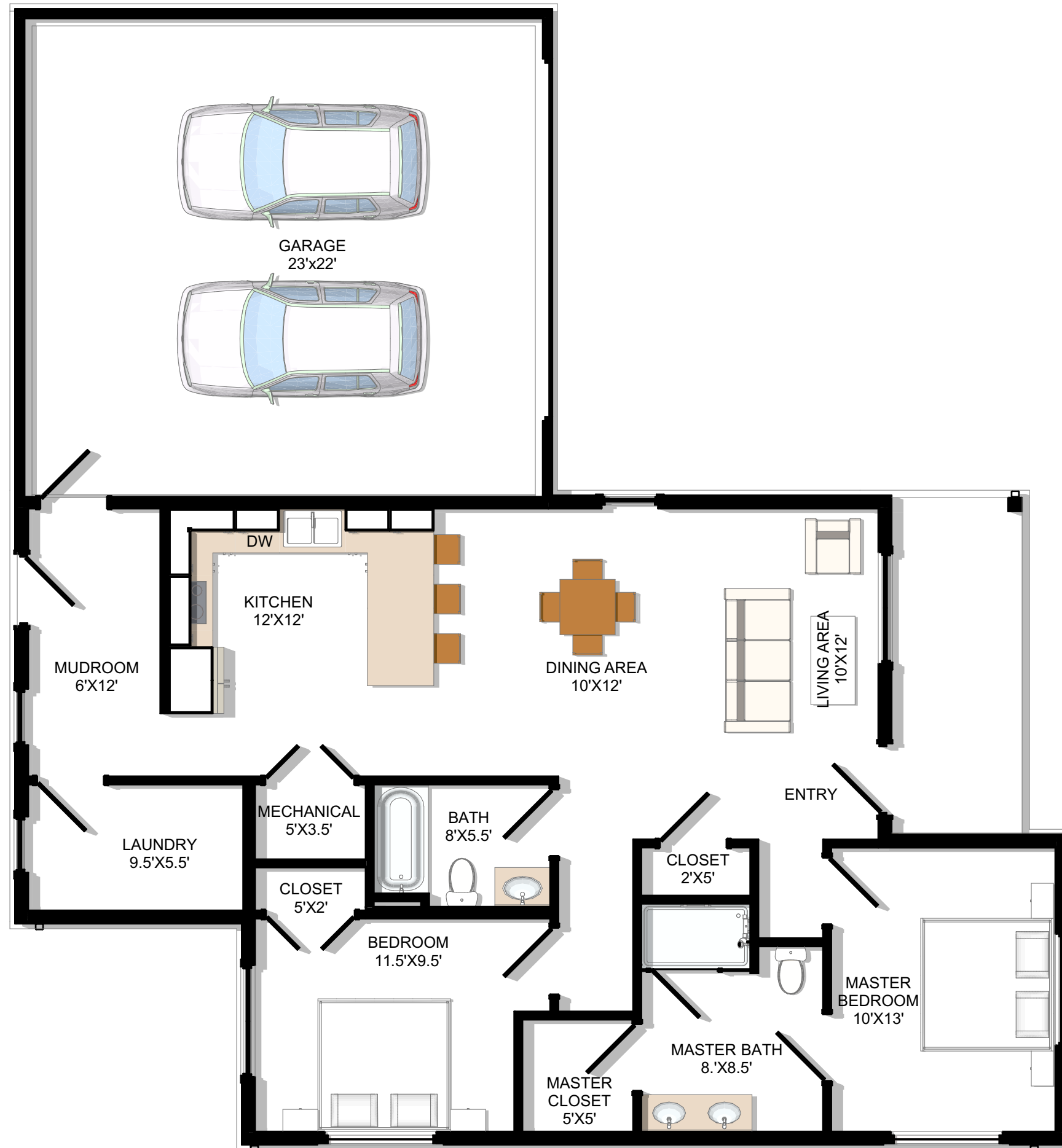
The Minimalist- FIRST FLOOR- 2 CAR FOUNDATION OPTION
