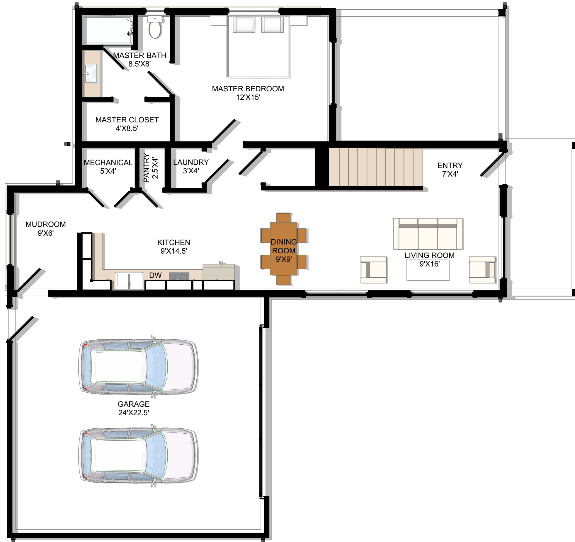
THE TWO YEAR OLD- FIRST FLOOR - FOUNDATION OPTION
