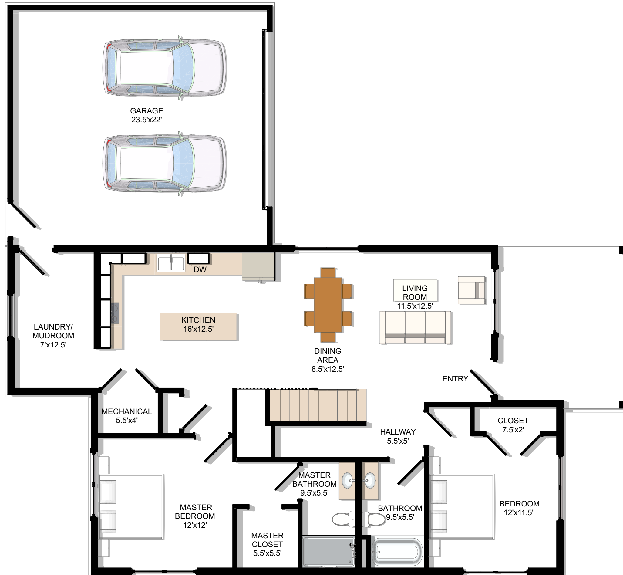
The Lemonade- FIRST FLOOR- FOUNDATION OPTION
